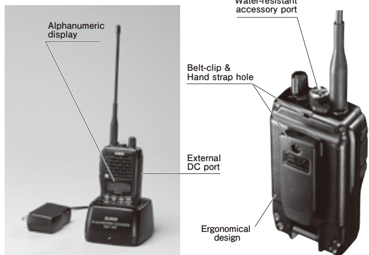
with optional Li-ion charger (E-version standard)
