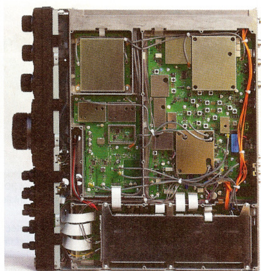
FTDX5000 underneath view with covers removed showing the main RF boards and synthesisers.
